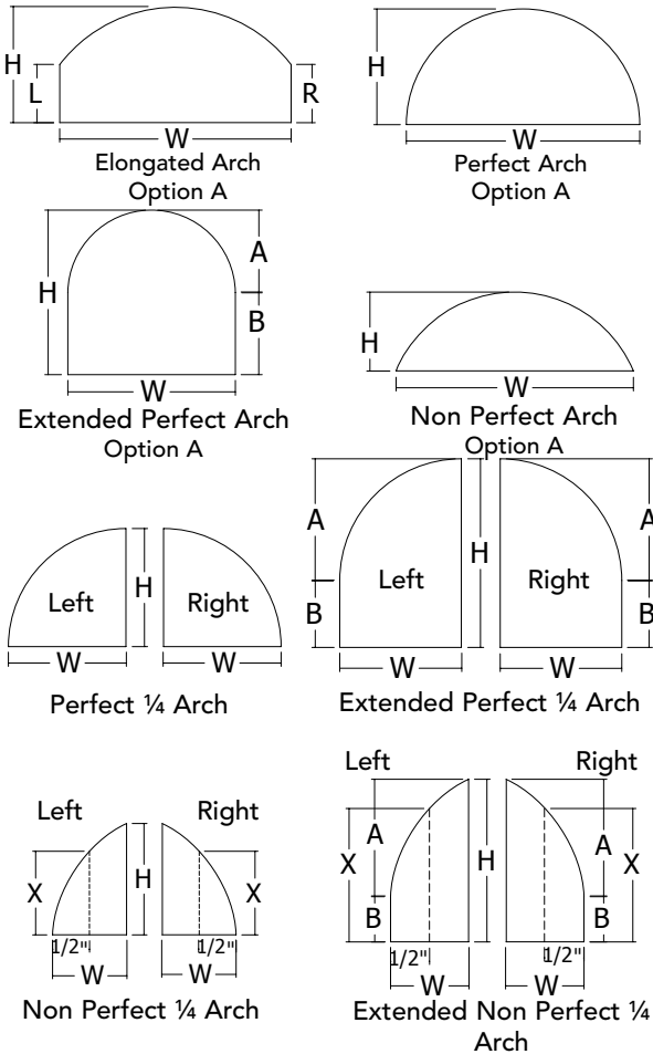
All Quarter Arches Left Side: Option F Right Side: Option G
